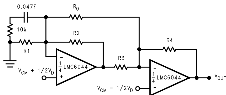
Figure 35. Two Op-Amp Instrumentation Amplifier
